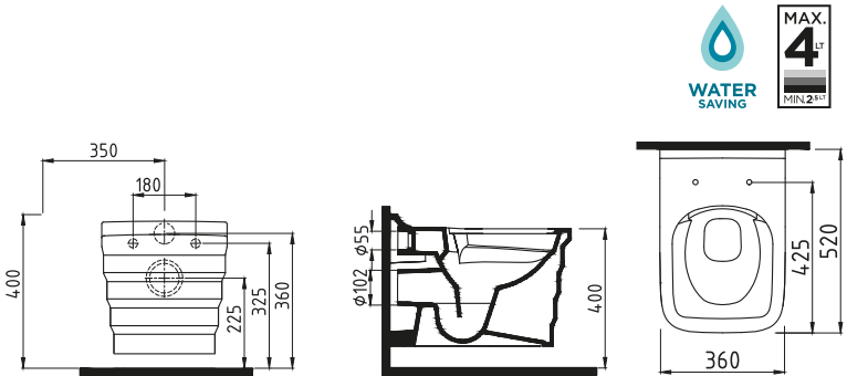
WALL HUNG WC PAN 52 cm NO-RIM/ CONCEALED FIXING SHKA052N1VPOW3000 520x360mm
