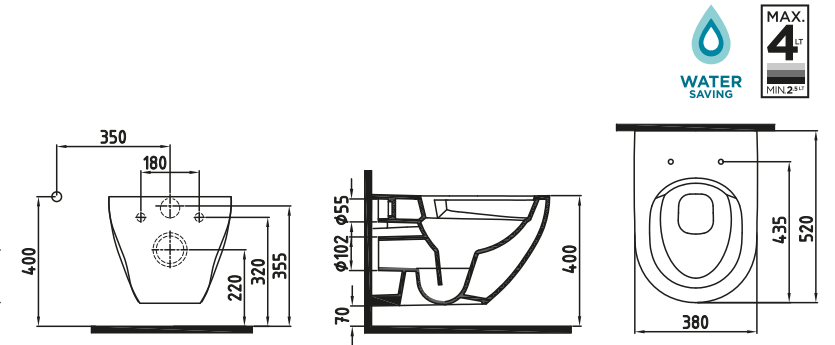
WALL HUNG WC PAN 52 cm NO-RIM/ CONCEALED FIXING DNKA052N1VP0W3000 520x380mm
