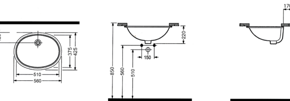
SINGLE PIECE UNDERCOUNTER WASHBASIN 50 cm WITHOUT HOLE TPLA05001VDOW3000
