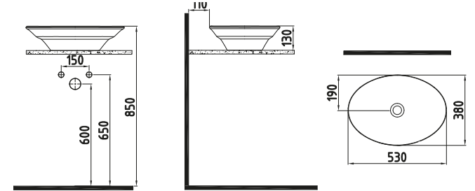
COUNTERTOP WASHBASIN 53 cm WITHOUT HOLE DNLG05301FDOW5000 530x380mm
