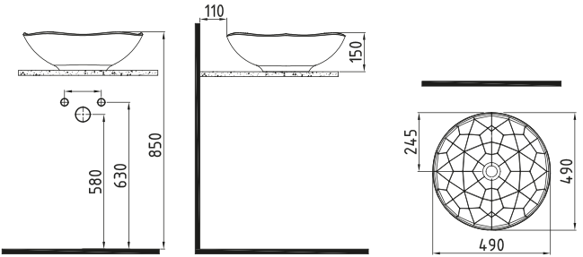
COUNTERTOP WASHBASIN 49 cm WITHOUT HOLE PNLG04901FD0W5000 Ø490mm
