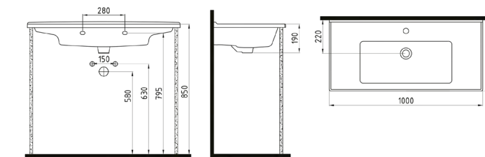
VANITY WASHBASIN 100 cm SINGLE HOLE NPLK10001FD1W5000 1000x470mm
