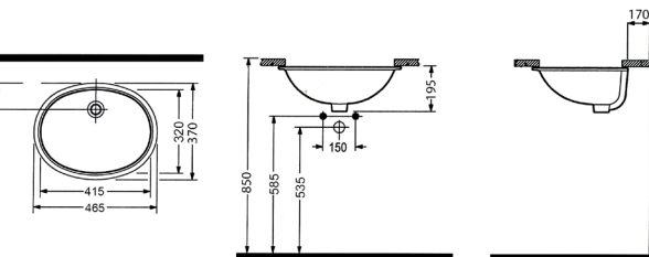
SINGLE PIECE UNDERCOUNTER WASHBASIN 41 cm WITHOUT HOLE TPLA04101VDOW3000
