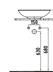
COUNTERTOP WASHBASIN 43 cm WITHOUT HOLE HRLG04301FD0W5000 430x430mm
