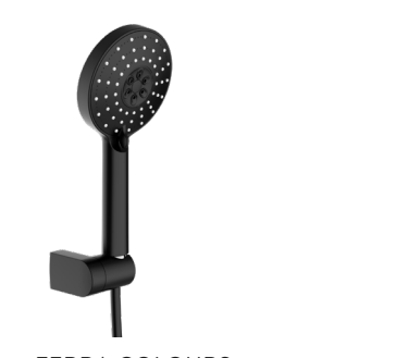
FERRA COLOURS SHOWER SET 3F BD14033512 Pieces In Box : 4 • 3 Function Hand Shower - Ø 120 mm • G 1/2" connection, 1.50 m Length-Black PVC Hose • Adjustable Shower Holder
