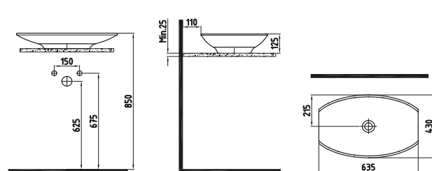
COUNTERTOP WASHBASIN 63 cm WITHOUT HOLE HRLG06301FDOW5000 630x430mm
