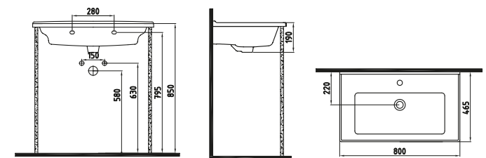
VANITY WASHBASIN 80 cm SINGLE HOLE NPLK08001FD1W5000 800x470mm
