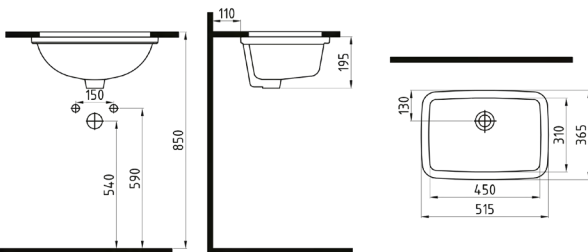
SINGLE PIECE UNDERCOUNTER WASHBASIN 45 cm WITHOUT HOLE TPLA04501VDOW3000
