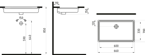
INFINITUM UNDERCOUNTER WASHBASIN 61 cm WITHOUT HOLE INLA06101FDOW5000
